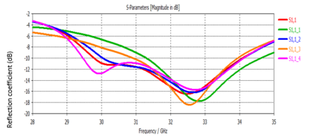
Figure 7. S11 parameter for all positions of L-slots
